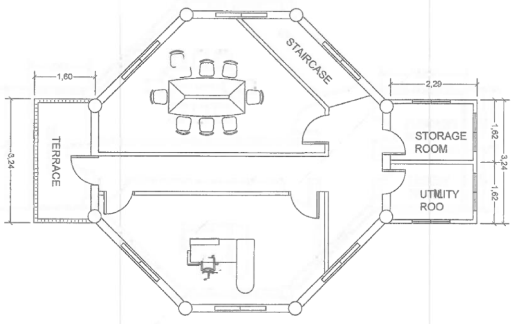
2 SECOND FLOOR PLAN SCALE: NTS
